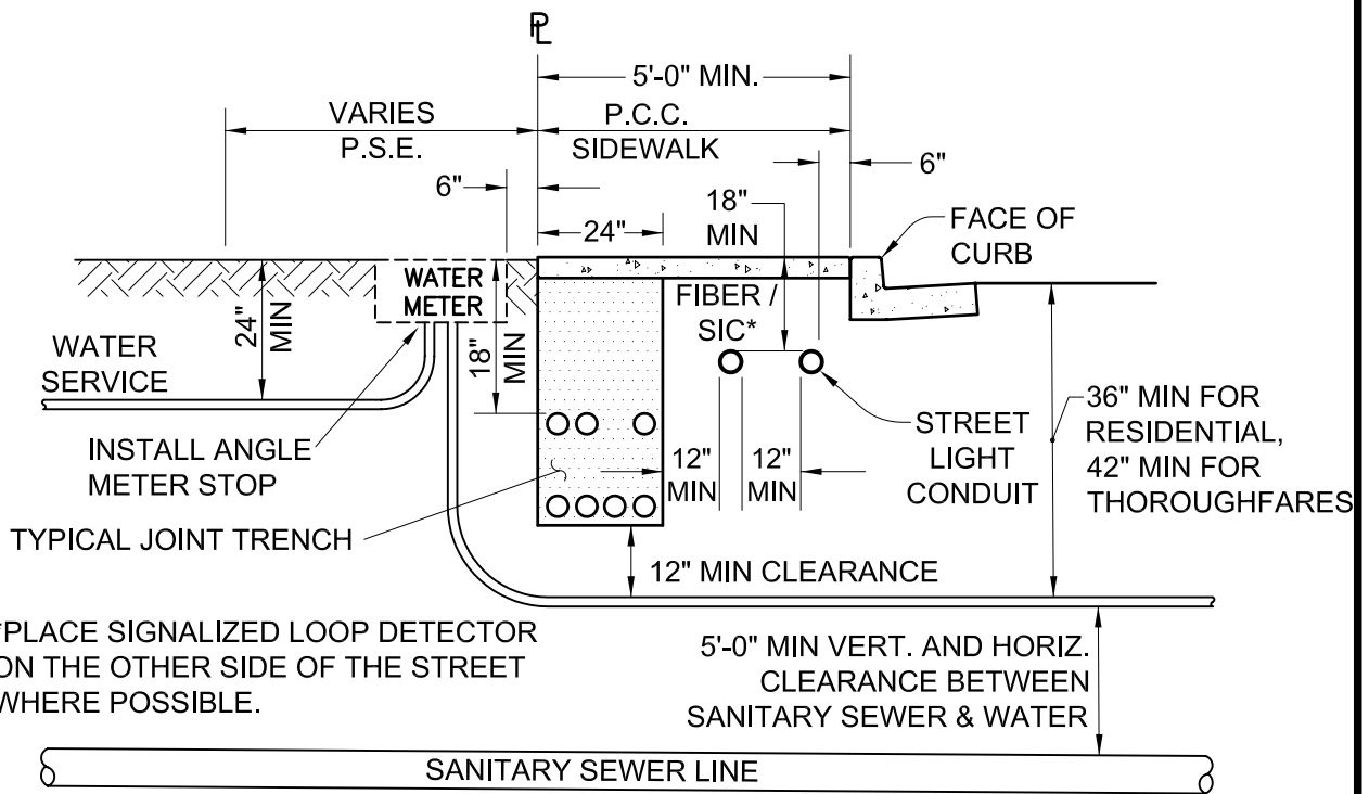
JOINT TRENCH DETAIL FOR MONOLITHIC SIDEWALK
