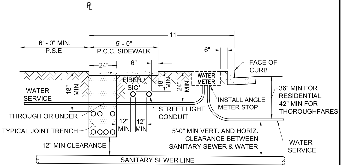
JOINT TRENCH DETAIL FOR SIDEWALK W/ PLANTER AREA
