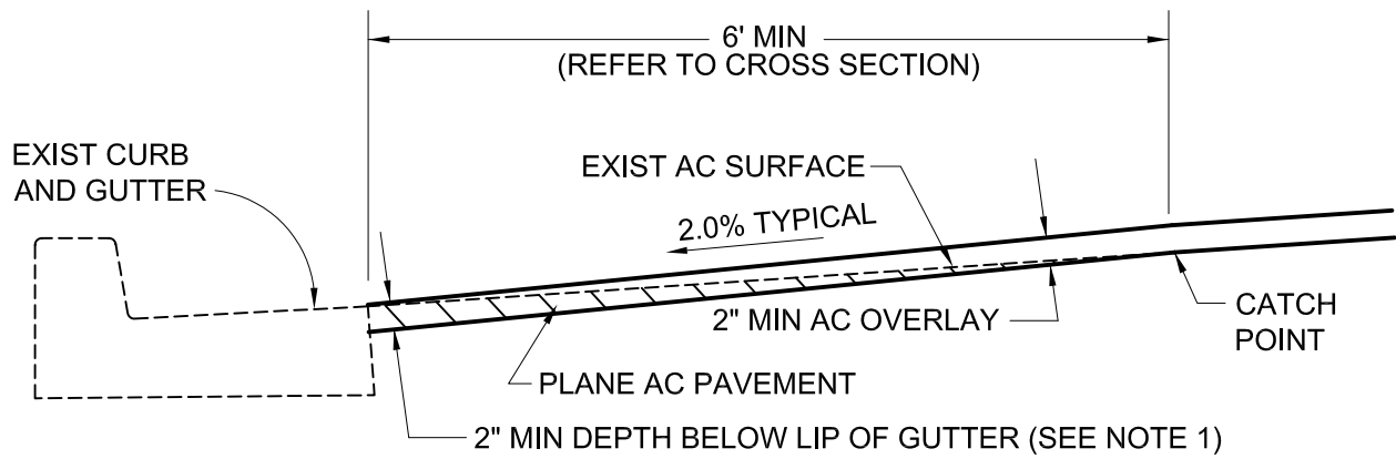
PLANNED PAVEMENT AT CURB AND GUTTER NO SCALE
