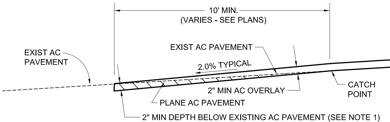
PLANNED PAVEMENT AT CURB AND GUTTER NO SCALE
